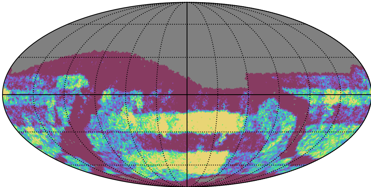
baseline_v3.5_10yrs Yr 3-4 r band: NVisits
