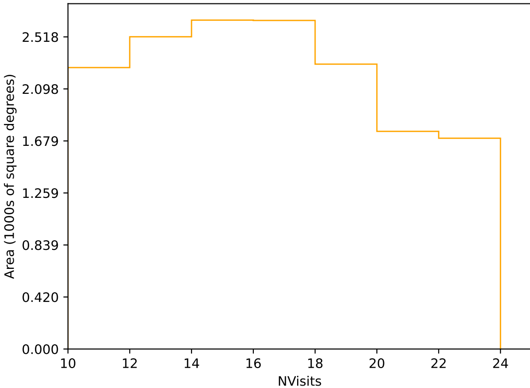
baseline_v3.5_10yrs Yr 3-4 r band: NVisits
