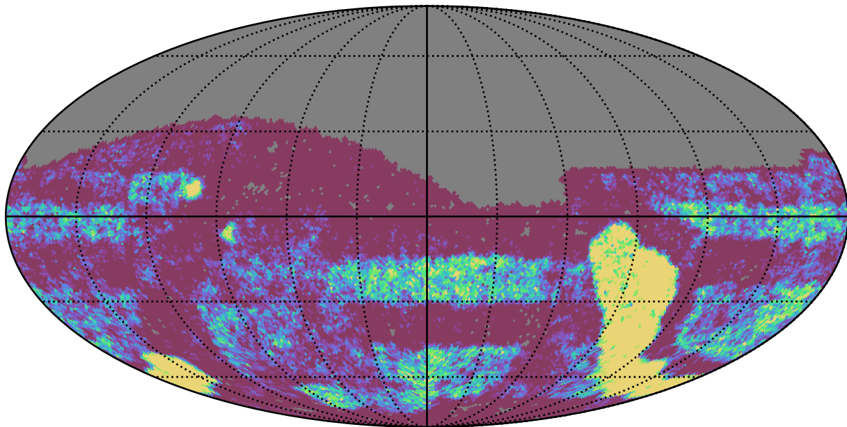
baseline_v3.5_10yrs Yr 3-4 g band: NVisits
