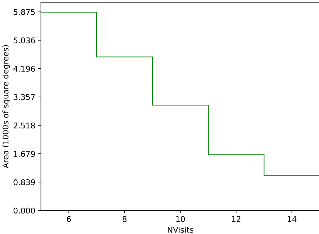
baseline_v3.5_10yrs Yr 3-4 g band: NVisits
