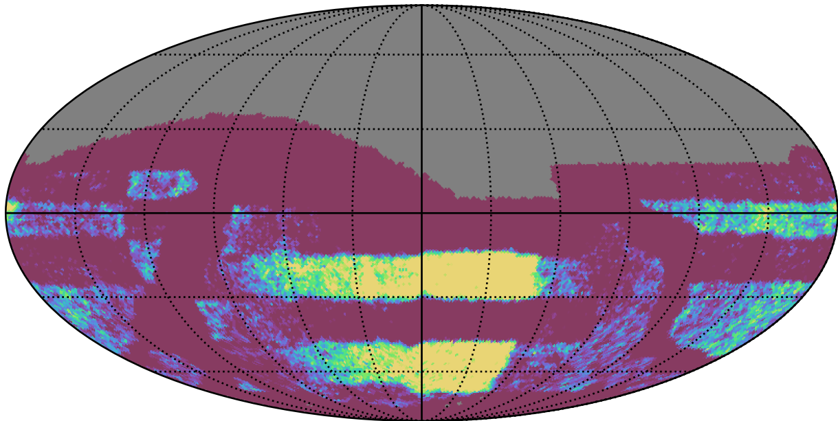
baseline_v3.5_10yrs Yr 3-4 all bands: NVisits
