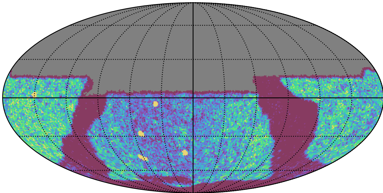
baseline_v3.5_10yrs Yr 1 y band: NVisits
