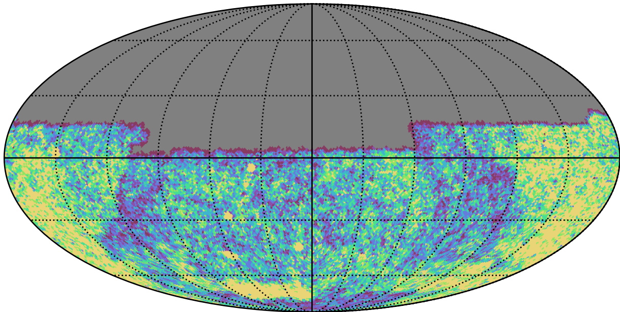
baseline_v3.5_10yrs Yr 1 u band: NVisits
