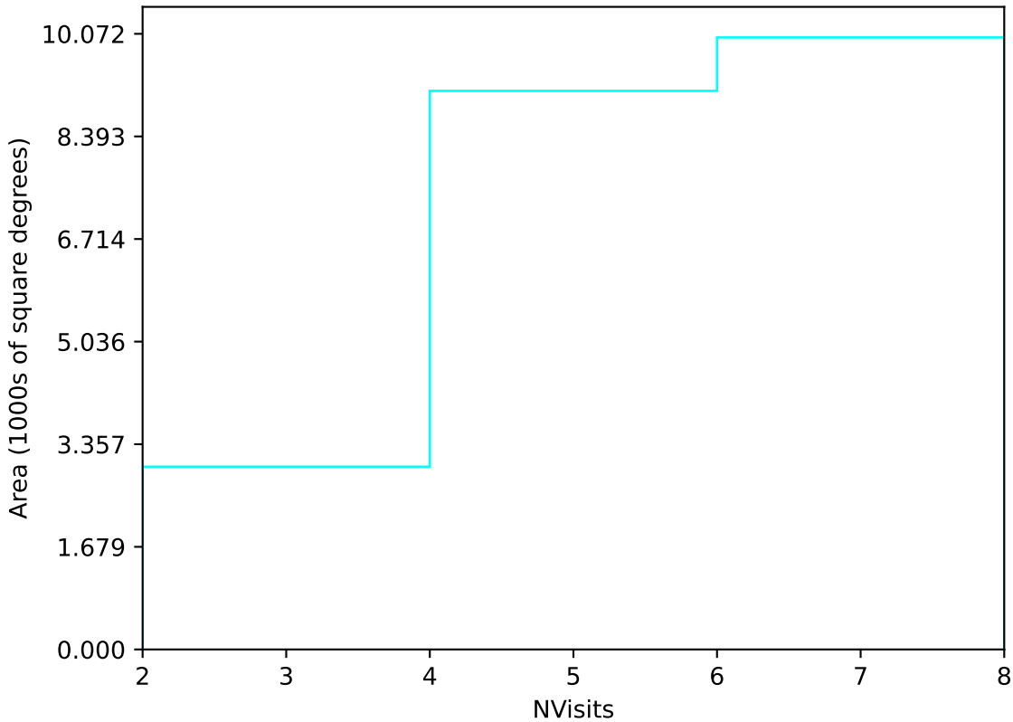
baseline_v3.5_10yrs Yr 1 u band: NVisits
