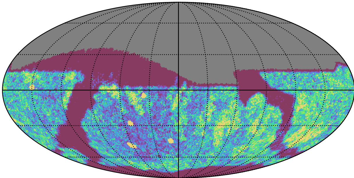
baseline_v3.5_10yrs Yr 1 r band: NVisits
