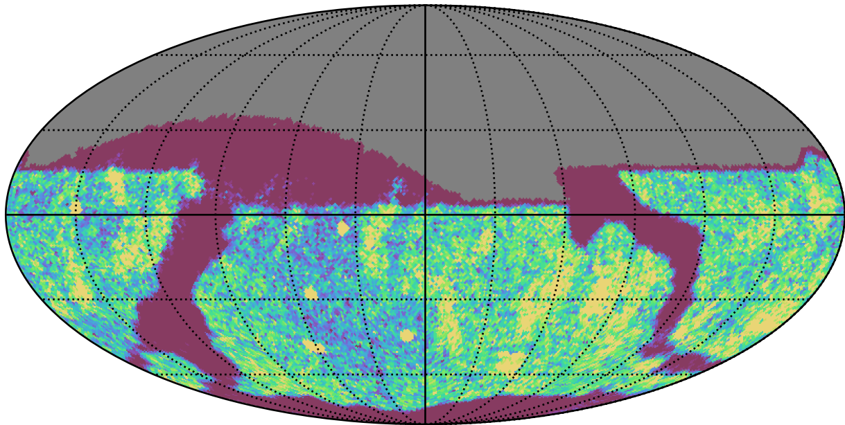
baseline_v3.5_10yrs Yr 1 i band: NVisits
