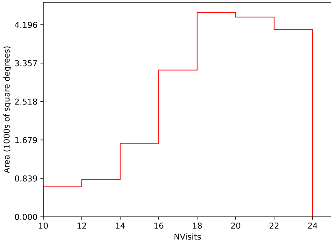
baseline_v3.5_10yrs Yr 1 i band: NVisits
