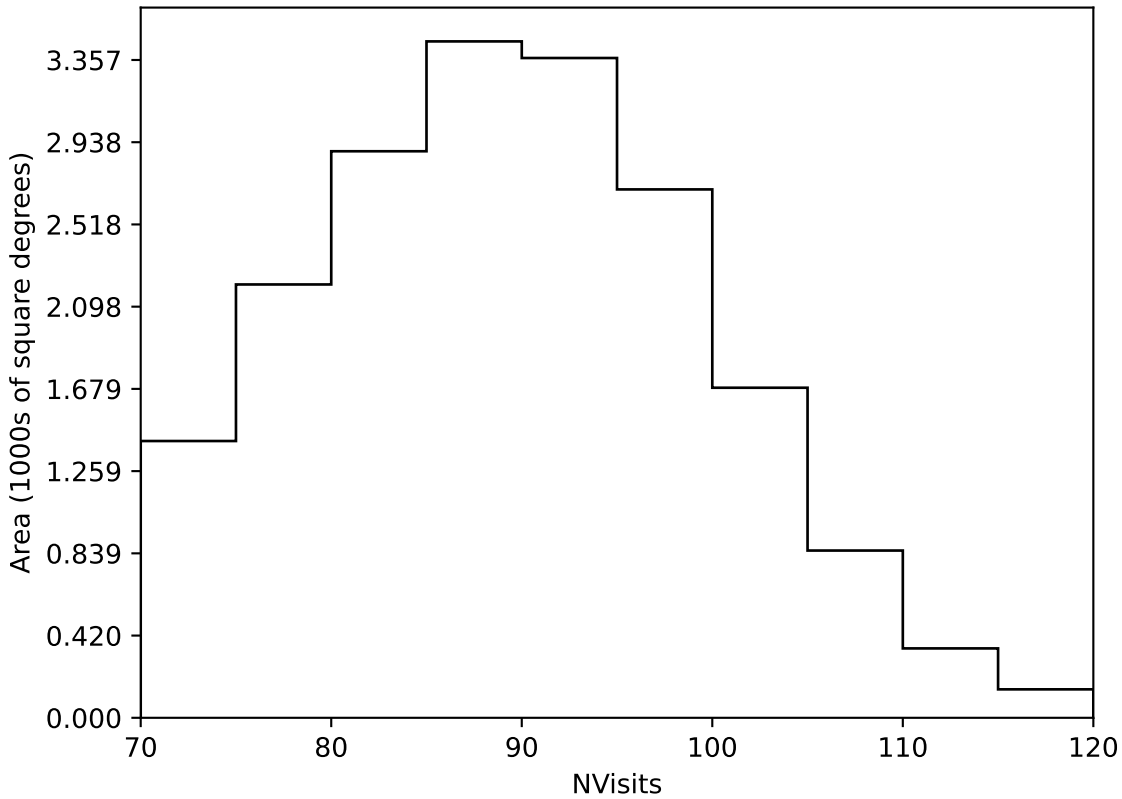
baseline_v3.5_10yrs Yr 1 all bands: NVisits
