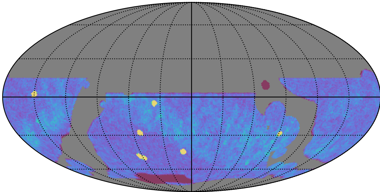
baseline_v3.5_10yrs WFD z band: NVisits
