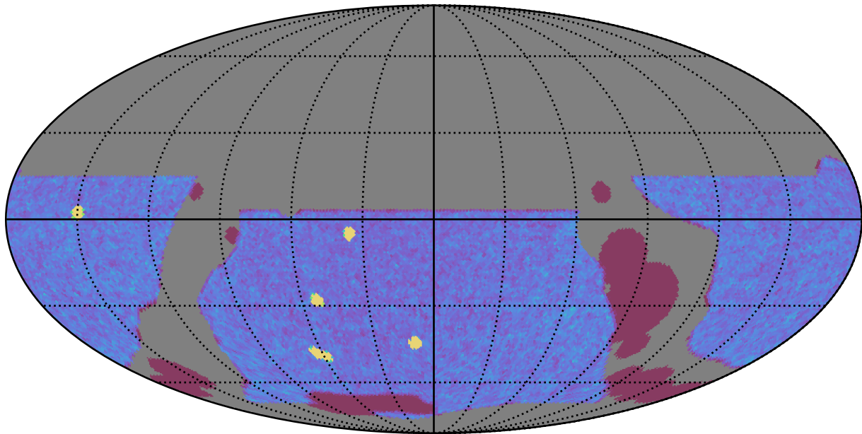
baseline_v3.5_10yrs WFD y band: NVisits
