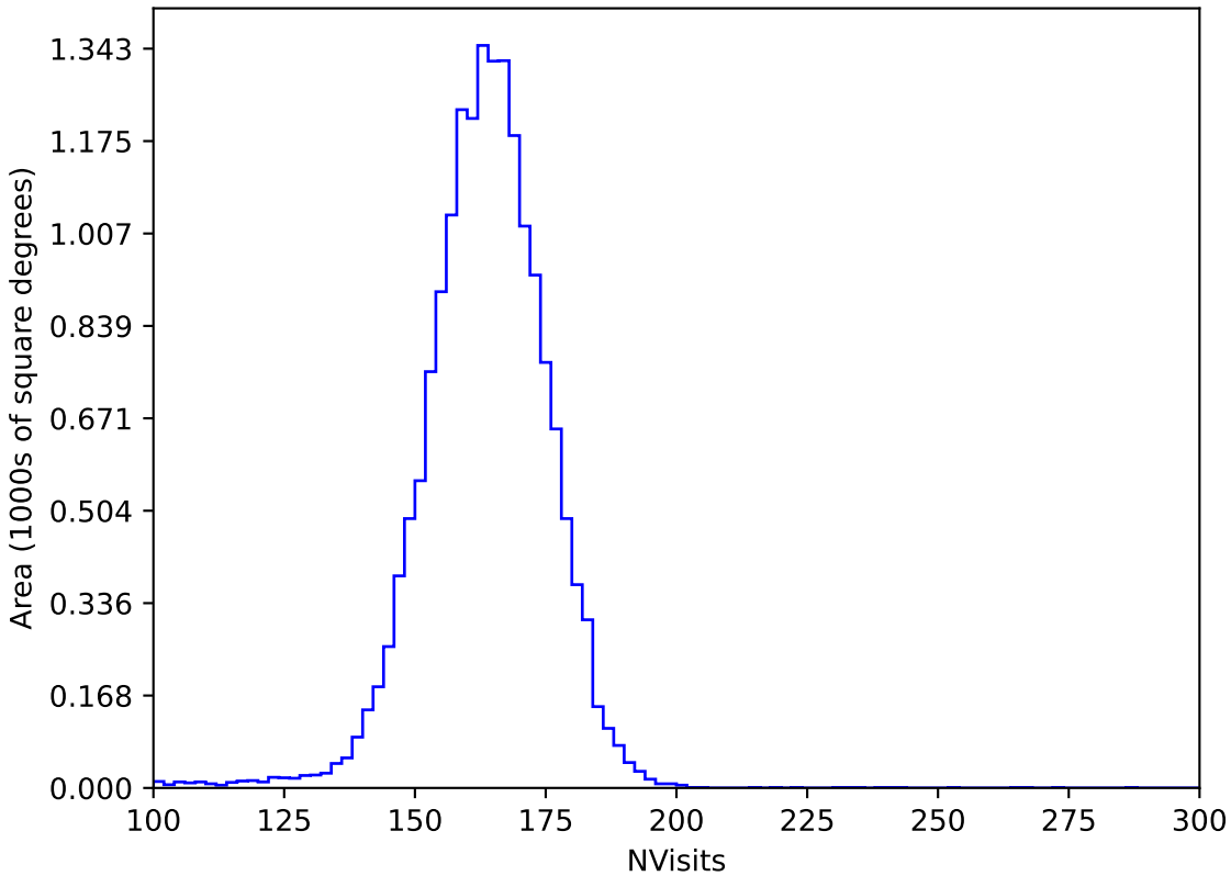
baseline_v3.5_10yrs WFD y band: NVisits
