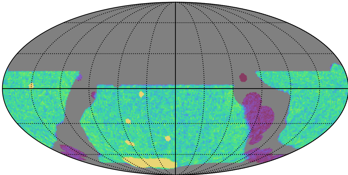
baseline_v3.5_10yrs WFD u band: NVisits
