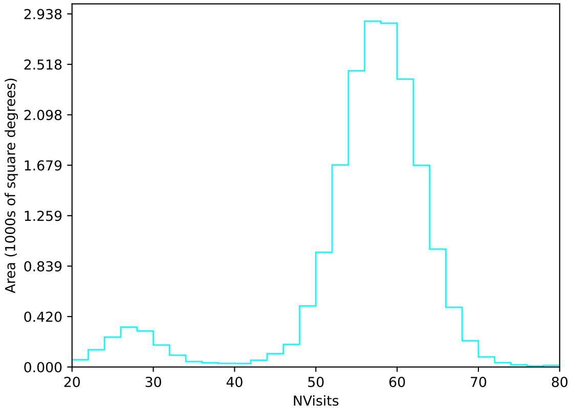
baseline_v3.5_10yrs WFD u band: NVisits
