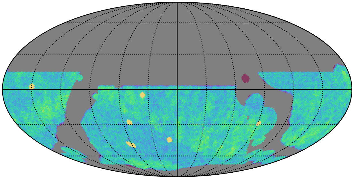
baseline_v3.5_10yrs WFD r band: NVisits
