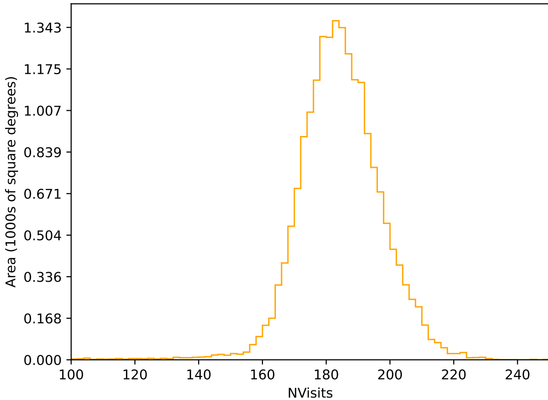
baseline_v3.5_10yrs WFD r band: NVisits
