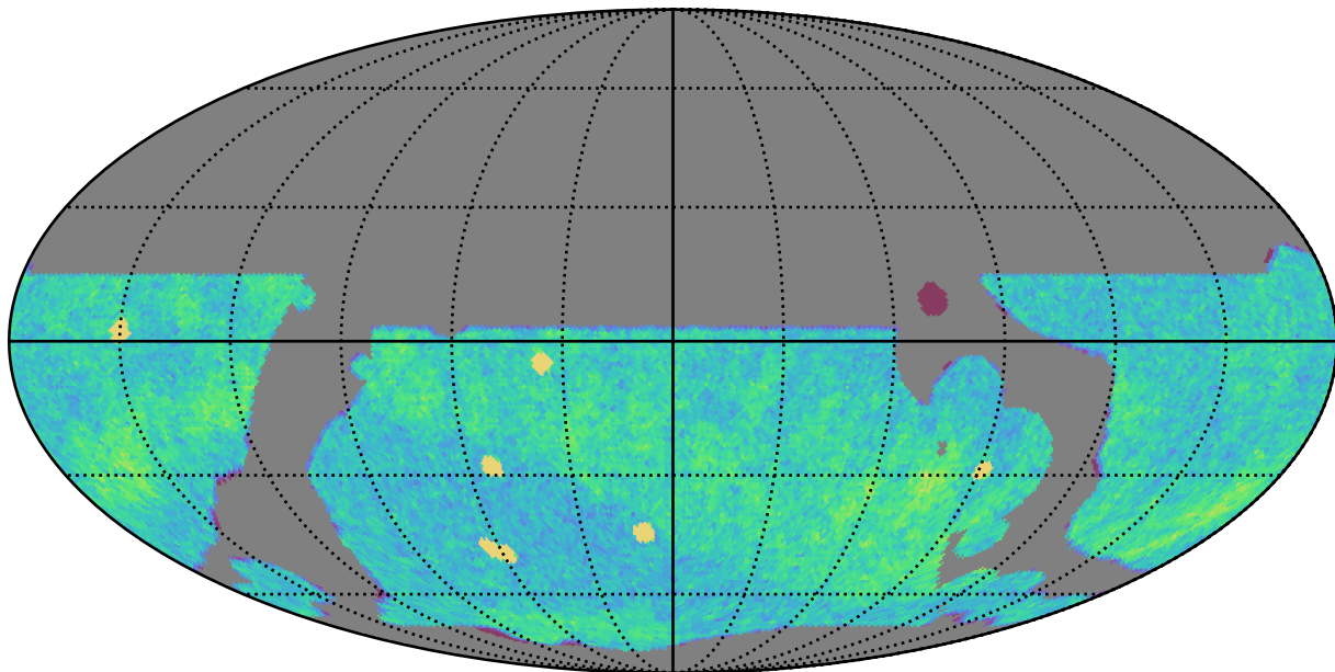
baseline_v3.5_10yrs WFD i band: NVisits
