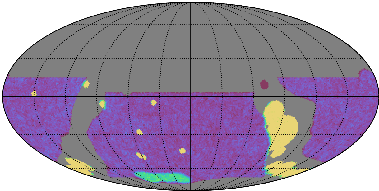
baseline_v3.5_10yrs WFD g band: NVisits
