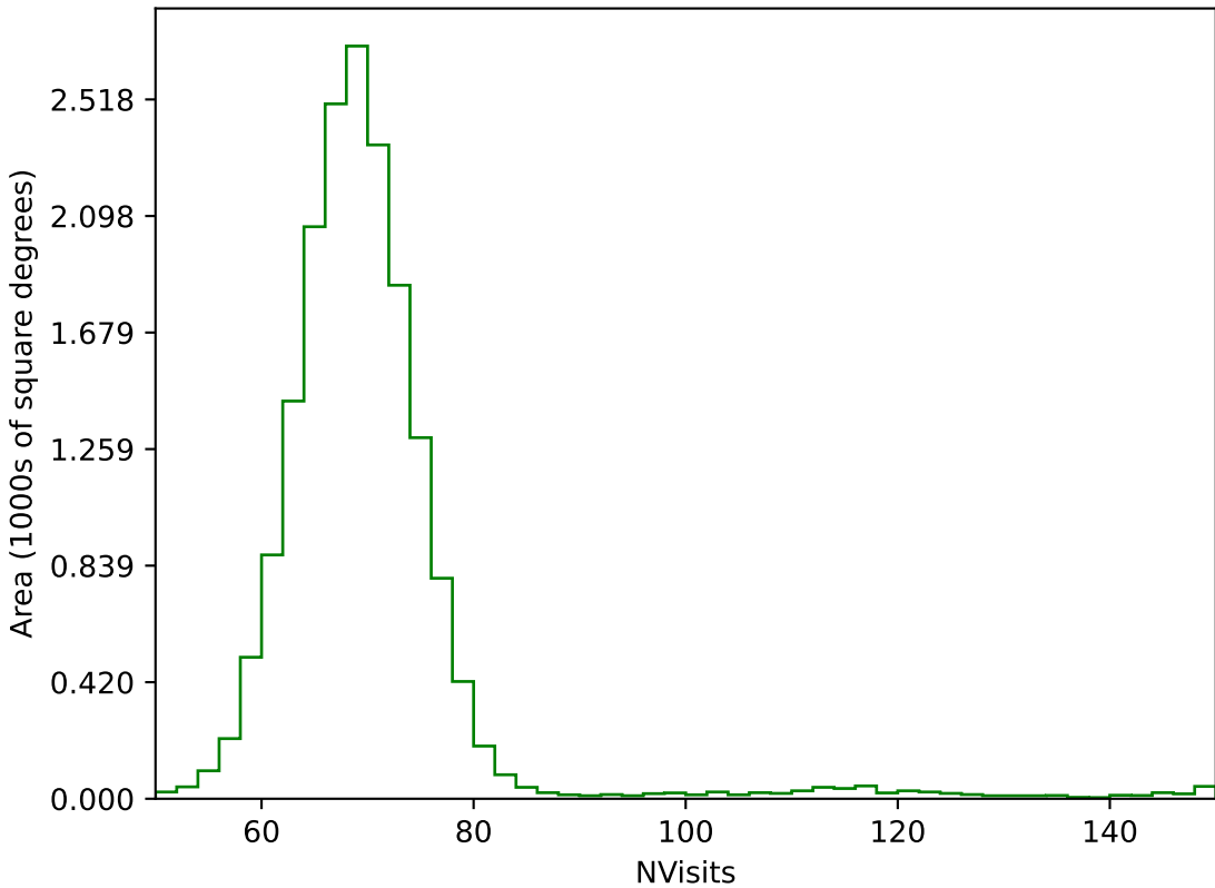
baseline_v3.5_10yrs WFD g band: NVisits
