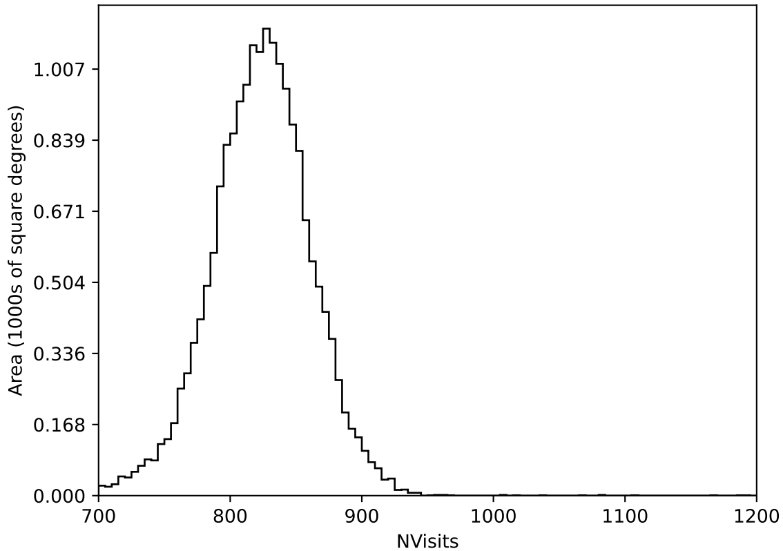
baseline_v3.5_10yrs WFD all bands: NVisits
