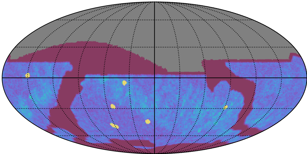
baseline_v3.5_10yrs All sky z band: NVisits
