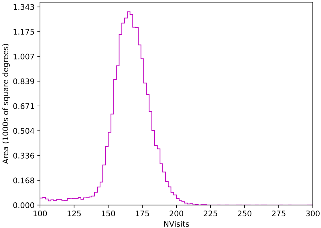
baseline_v3.5_10yrs All sky z band: NVisits
