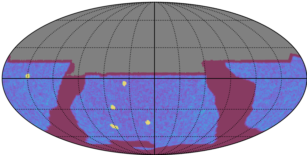
baseline_v3.5_10yrs All sky y band: NVisits
