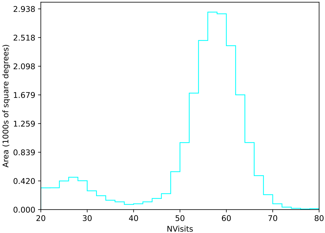
baseline_v3.5_10yrs All sky u band: NVisits
