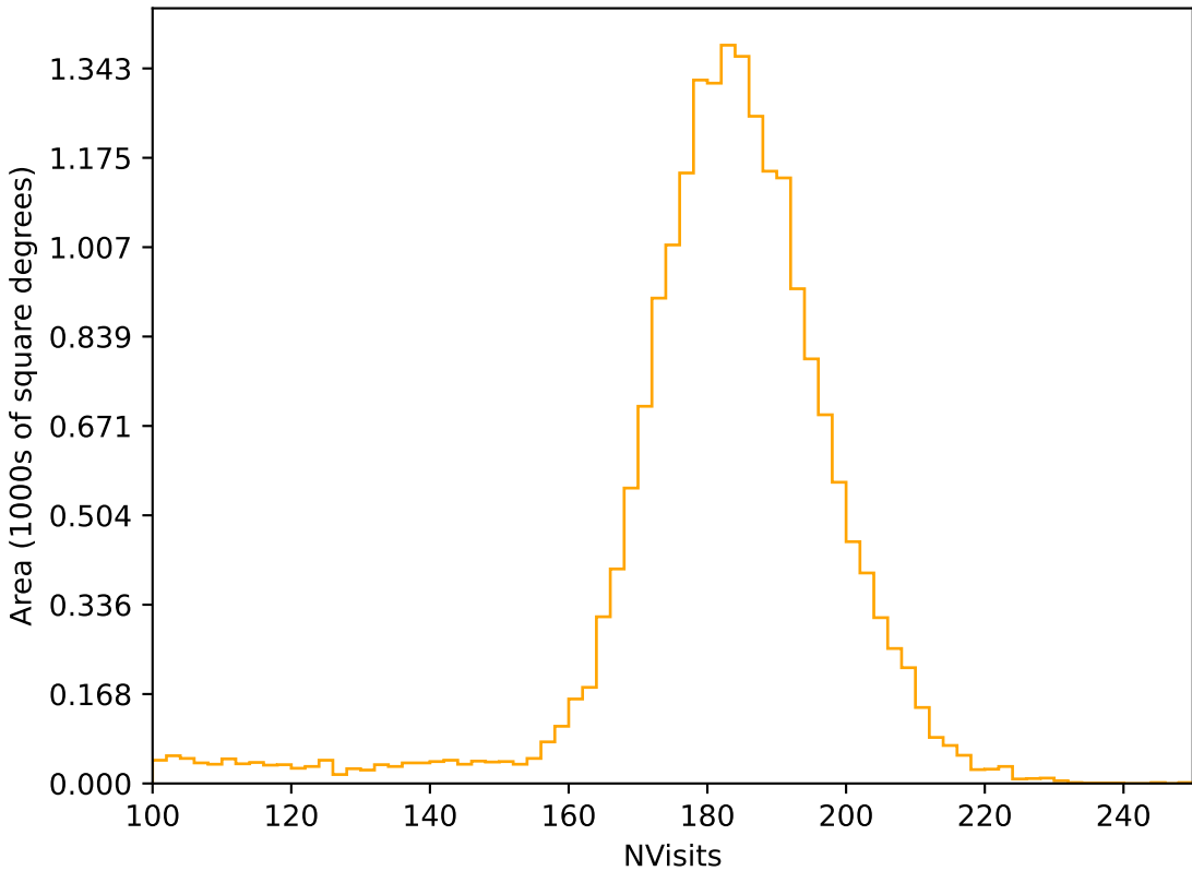
baseline_v3.5_10yrs All sky r band: NVisits
