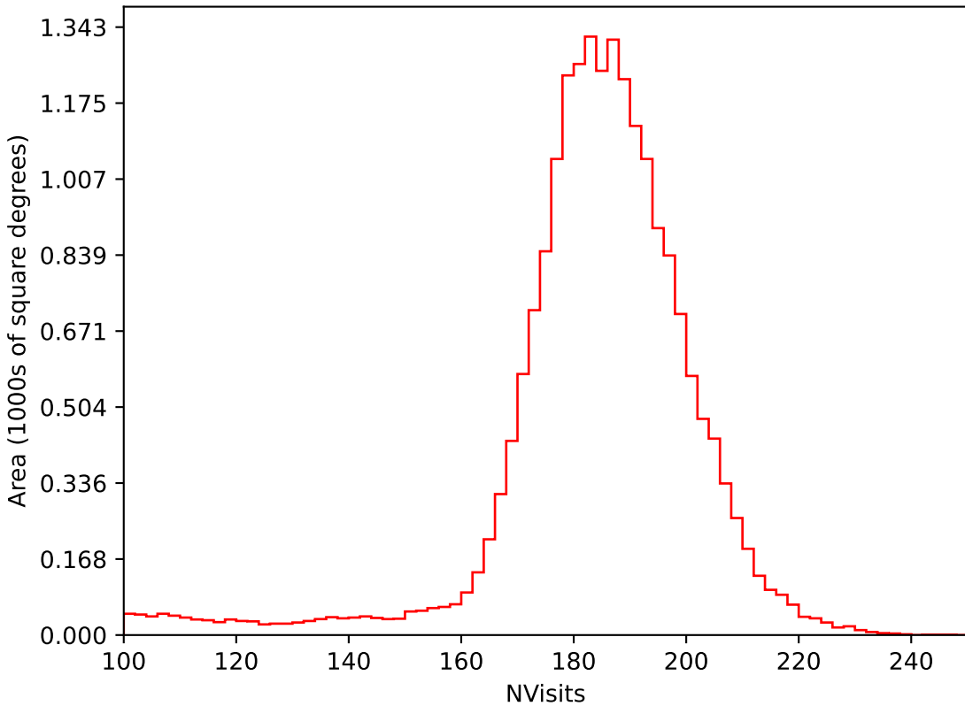
baseline_v3.5_10yrs All sky i band: NVisits
