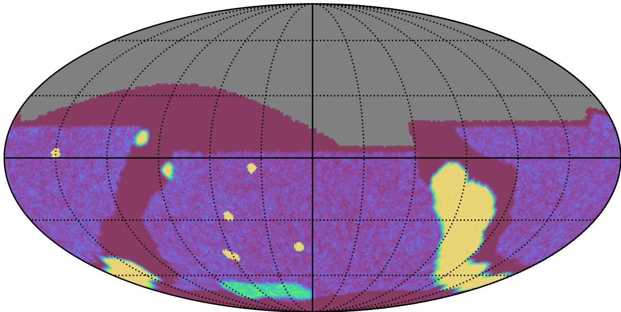
baseline_v3.5_10yrs All sky g band: NVisits
