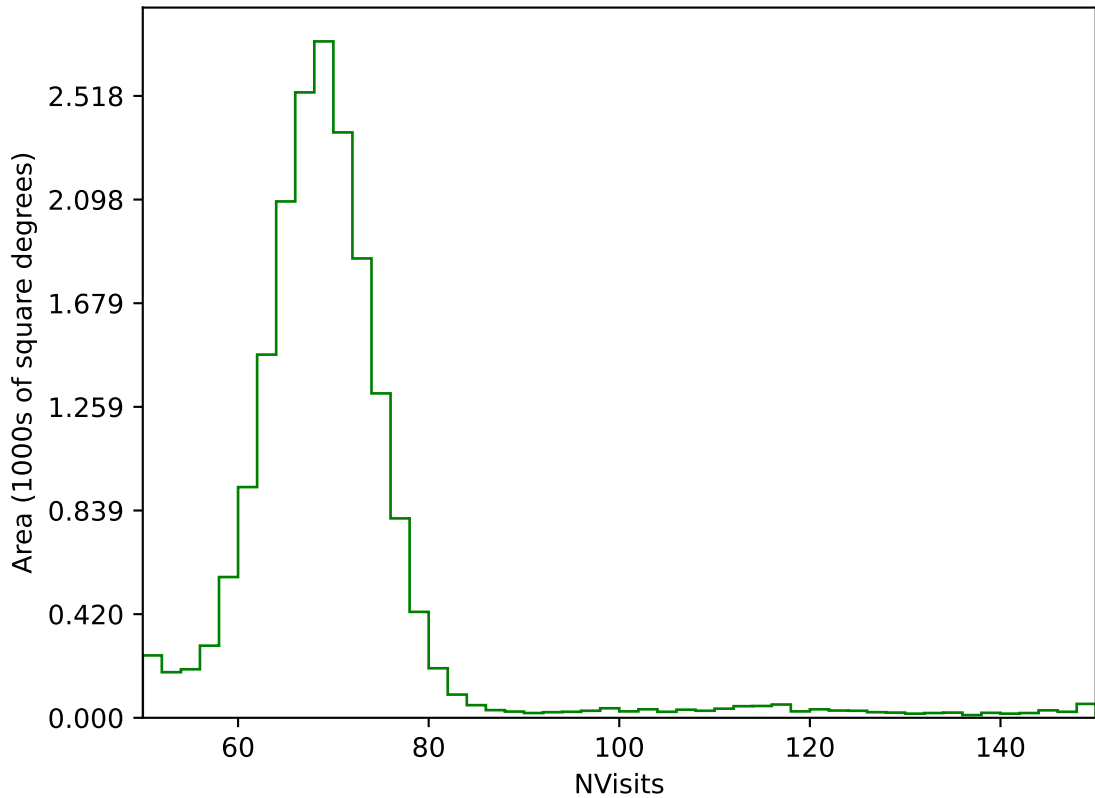
baseline_v3.5_10yrs All sky g band: NVisits
