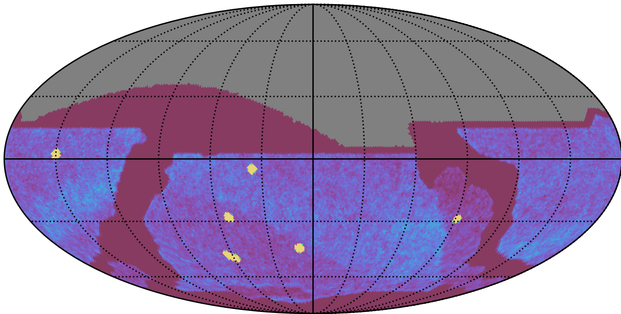
baseline_v3.5_10yrs All sky all bands: NVisits
