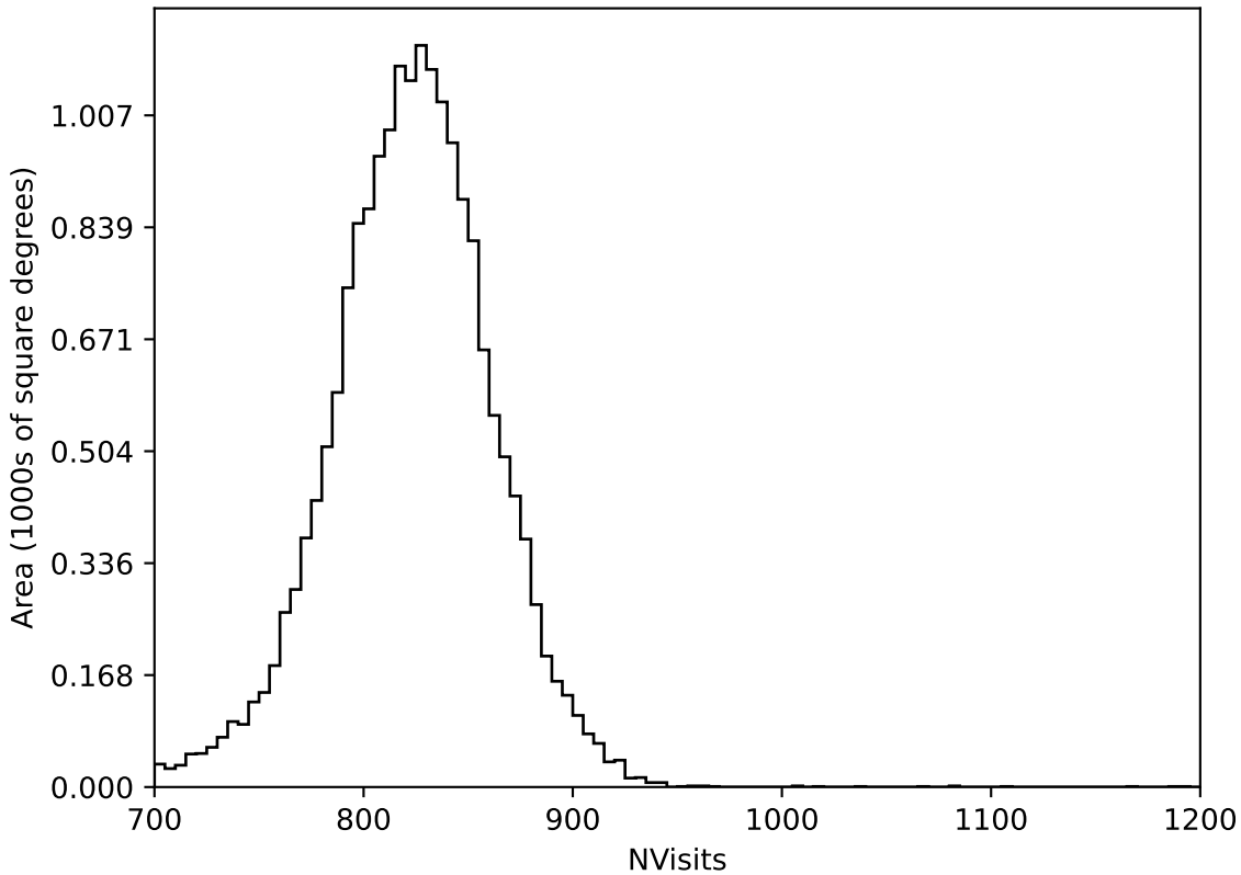
baseline_v3.5_10yrs All sky all bands: NVisits
