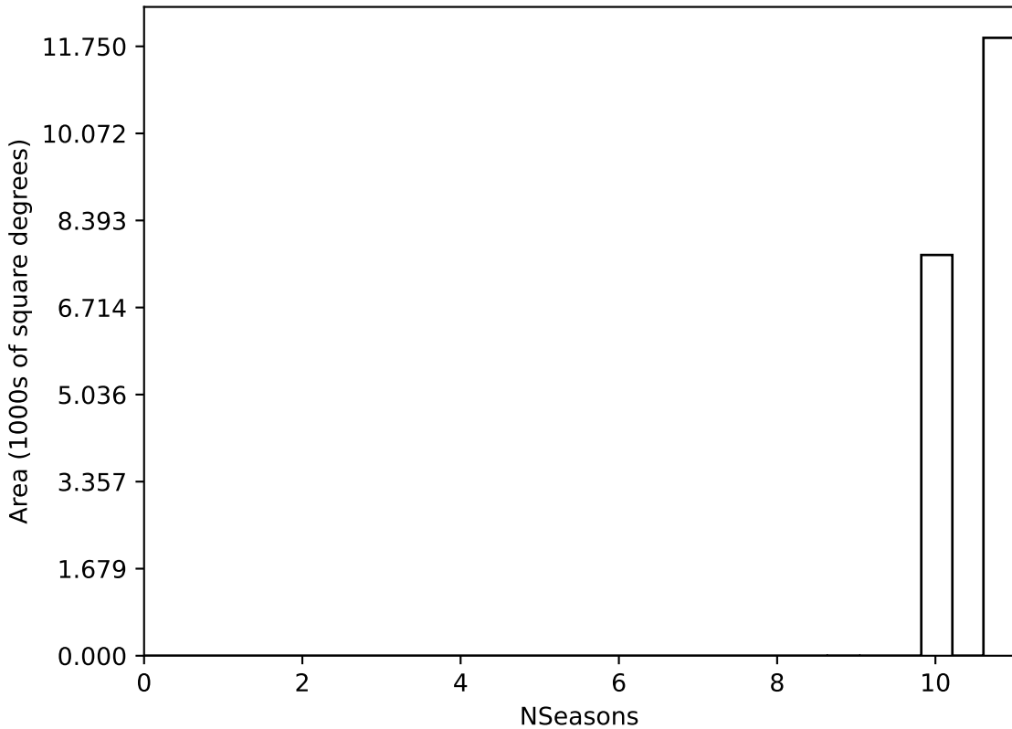
baseline_v3.5_10yrs WFD all bands: NSeasons
