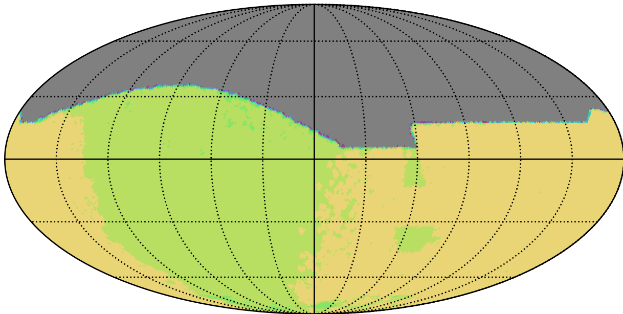
baseline_v3.5_10yrs All sky all bands: NSeasons
