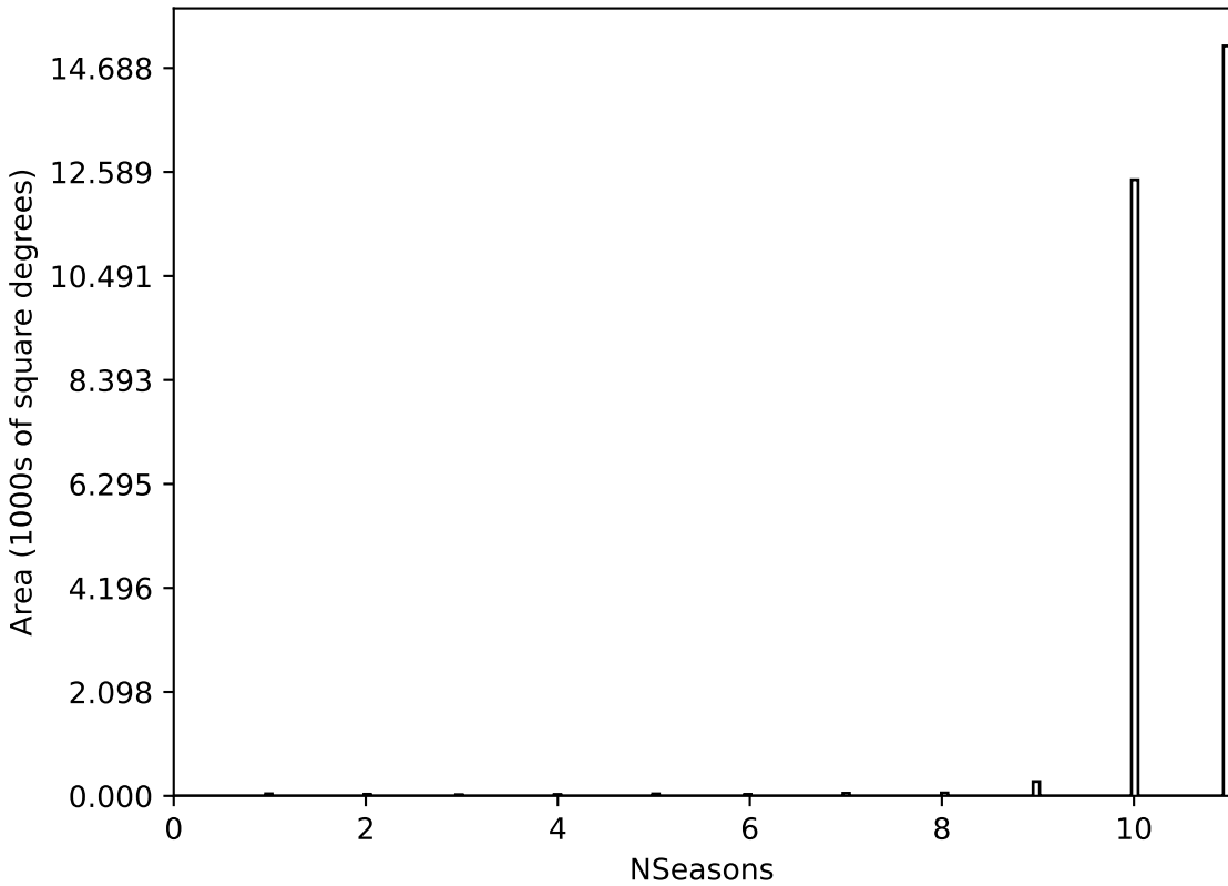
baseline_v3.5_10yrs All sky all bands: NSeasons
