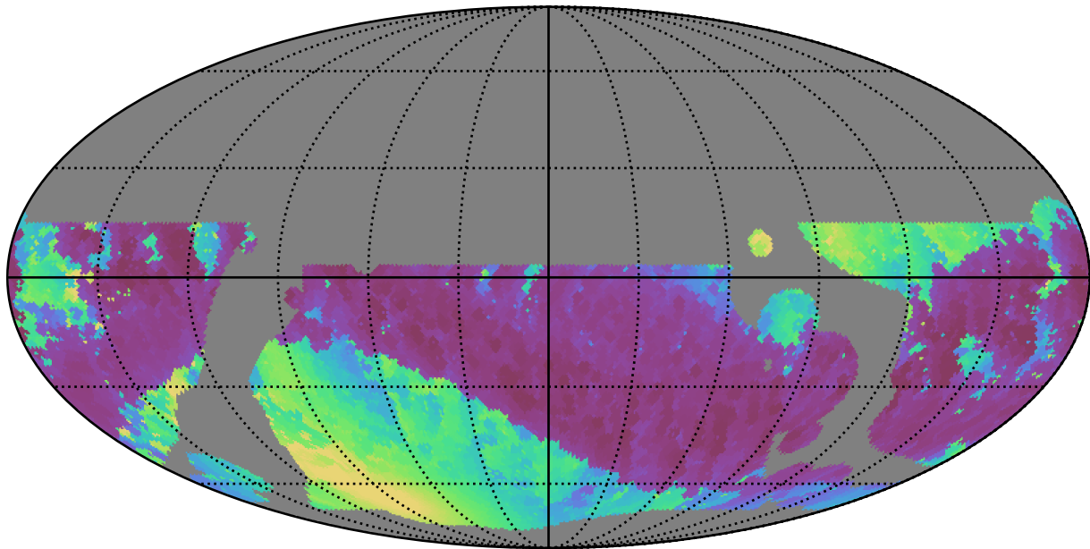
baseline_v3.5_10yrs WFD z band: Min solarElong
