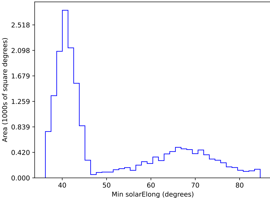
baseline_v3.5_10yrs WFD z band: Min solarElong
