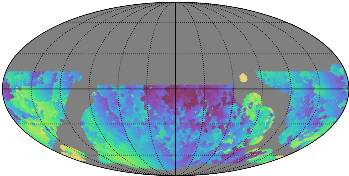
baseline_v3.5_10yrs WFD y band: Min solarElong
