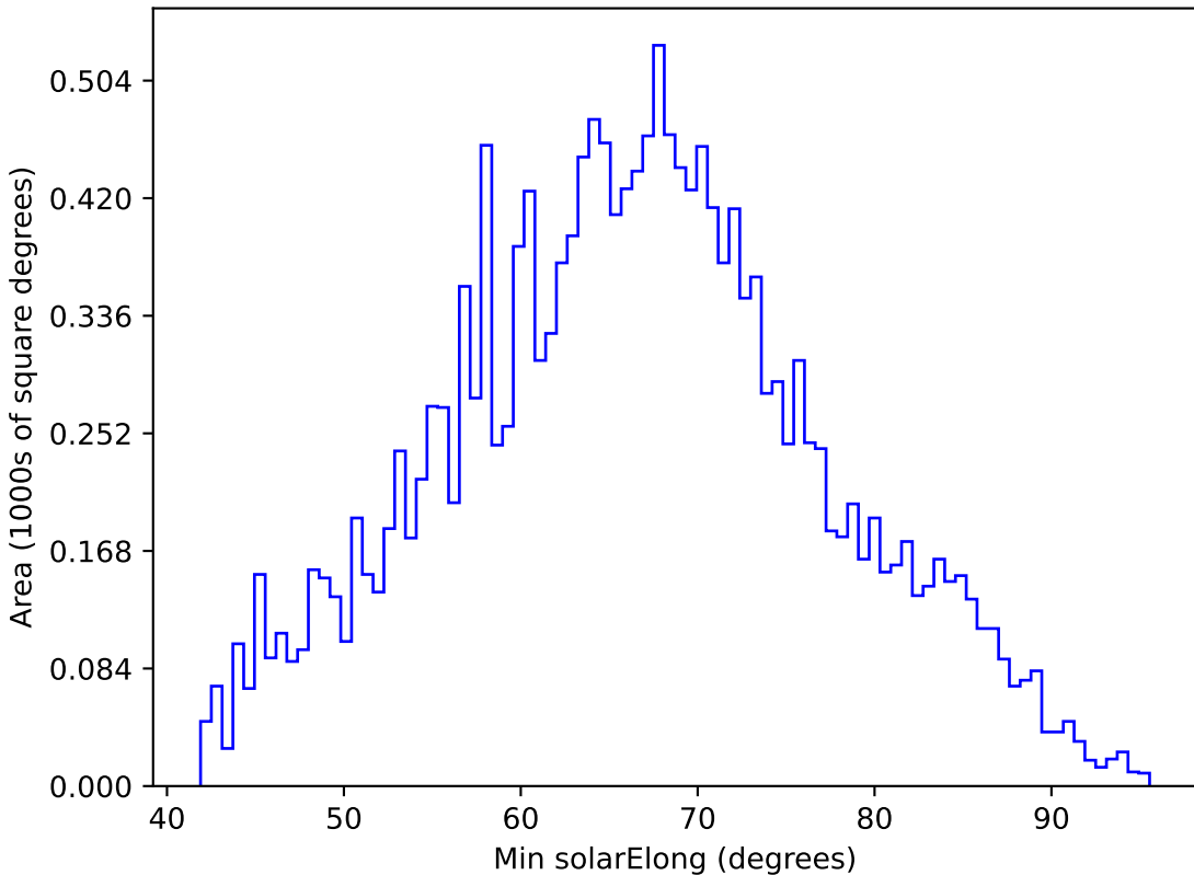
baseline_v3.5_10yrs WFD y band: Min solarElong
