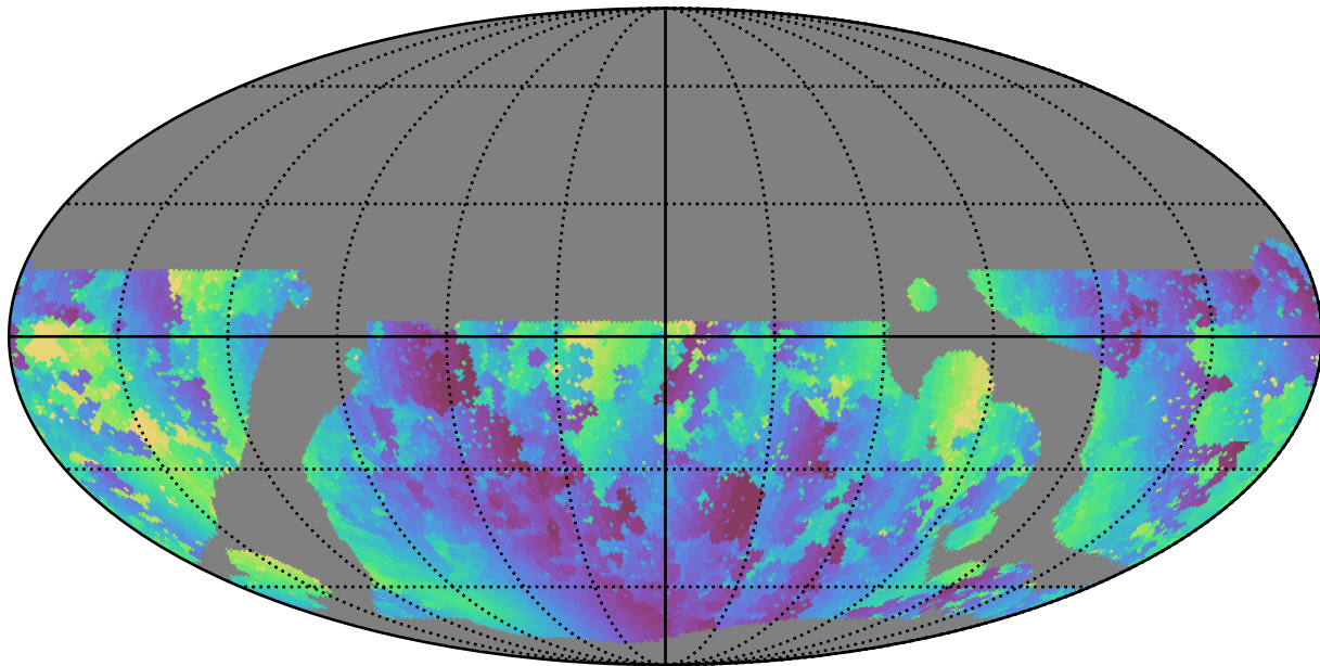
baseline_v3.5_10yrs WFD u band: Min solarElong
