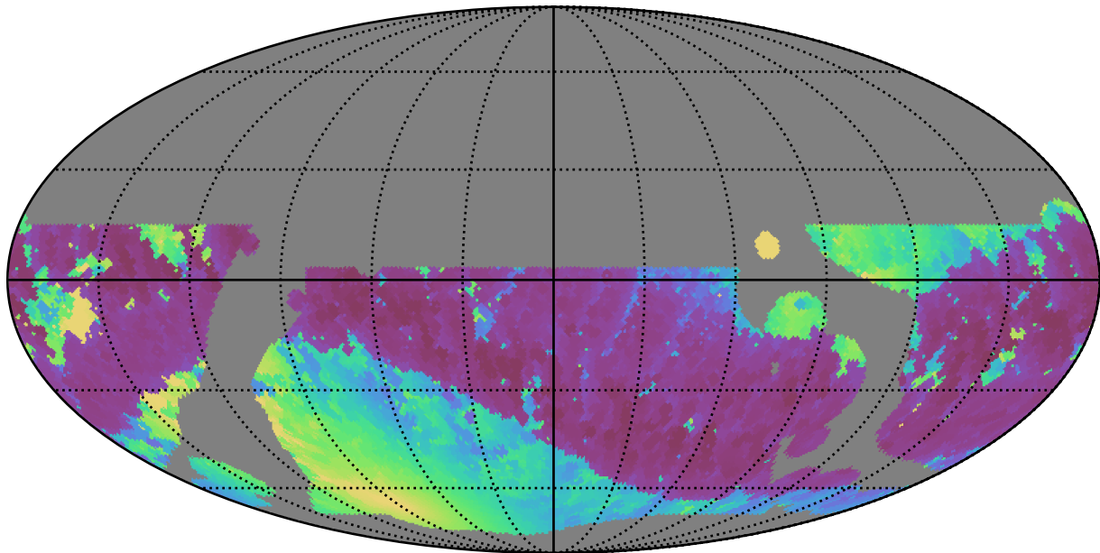
baseline_v3.5_10yrs WFD r band: Min solarElong
