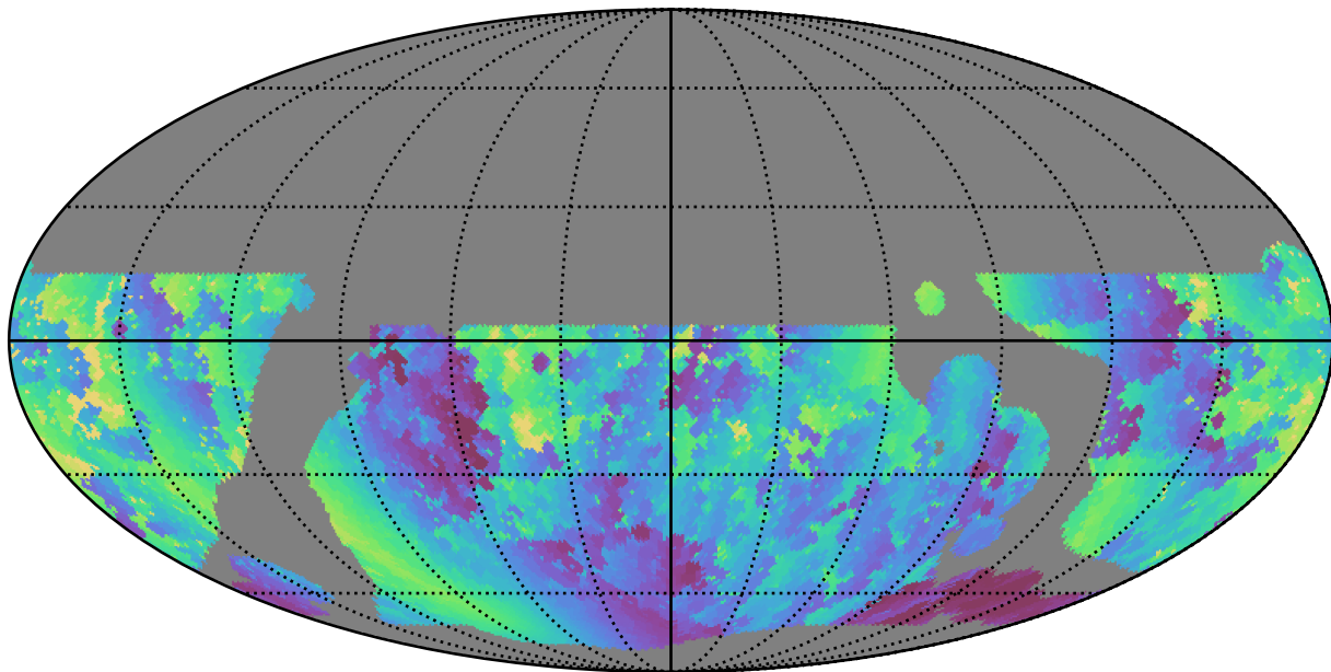
baseline_v3.5_10yrs WFD g band: Min solarElong
