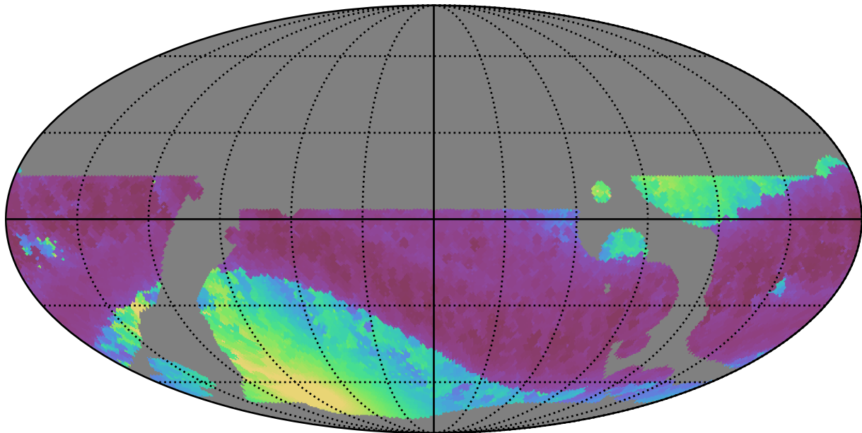
baseline_v3.5_10yrs WFD all bands: Min solarElong
