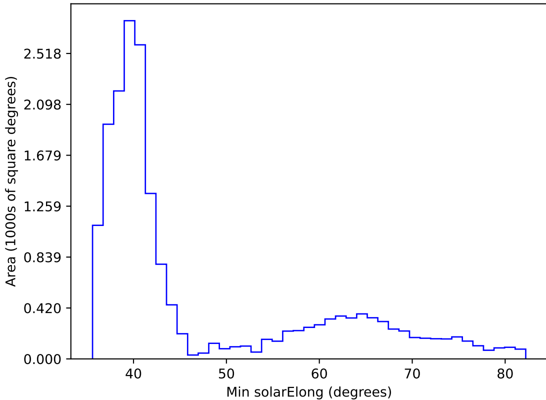
baseline_v3.5_10yrs WFD all bands: Min solarElong
