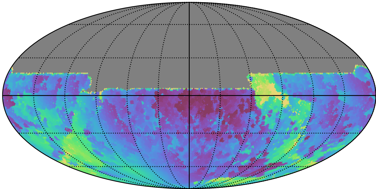
baseline_v3.5_10yrs All sky y band: Min solarElong
