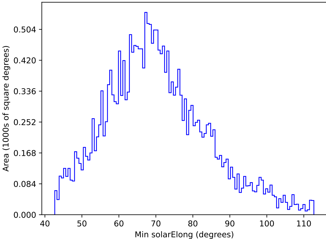
baseline_v3.5_10yrs All sky y band: Min solarElong
