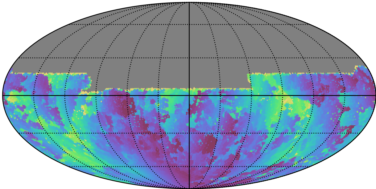
baseline_v3.5_10yrs All sky u band: Min solarElong
