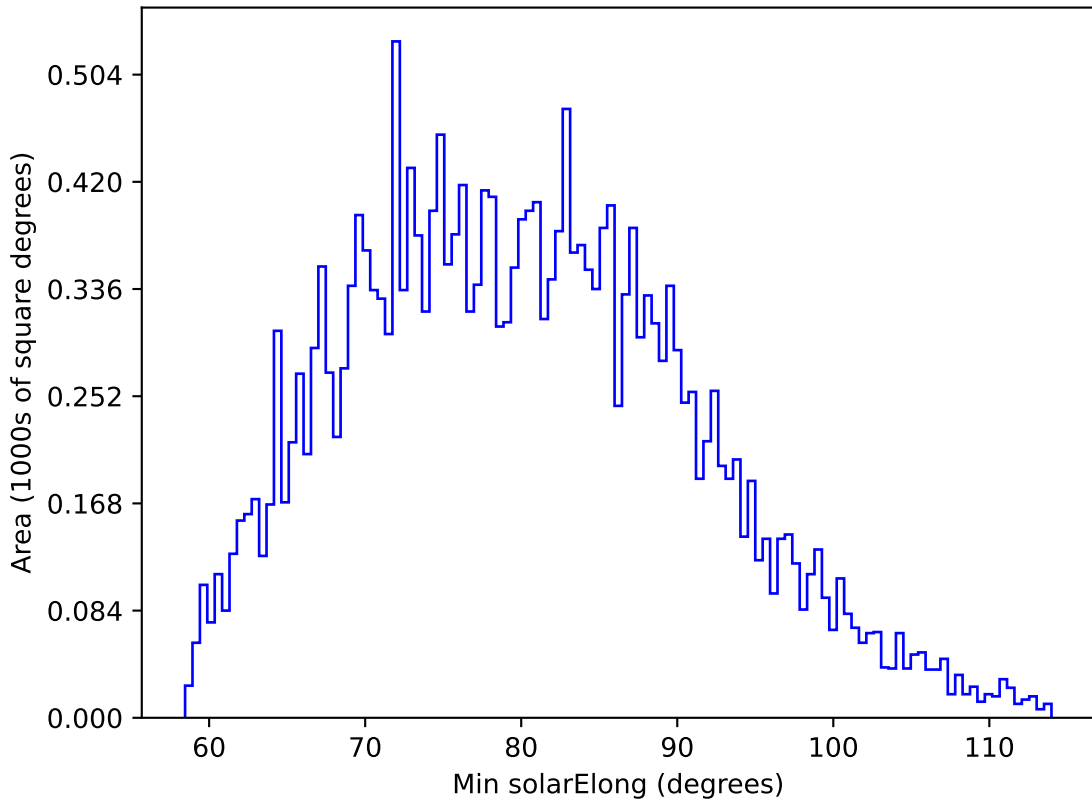
baseline_v3.5_10yrs All sky u band: Min solarElong
