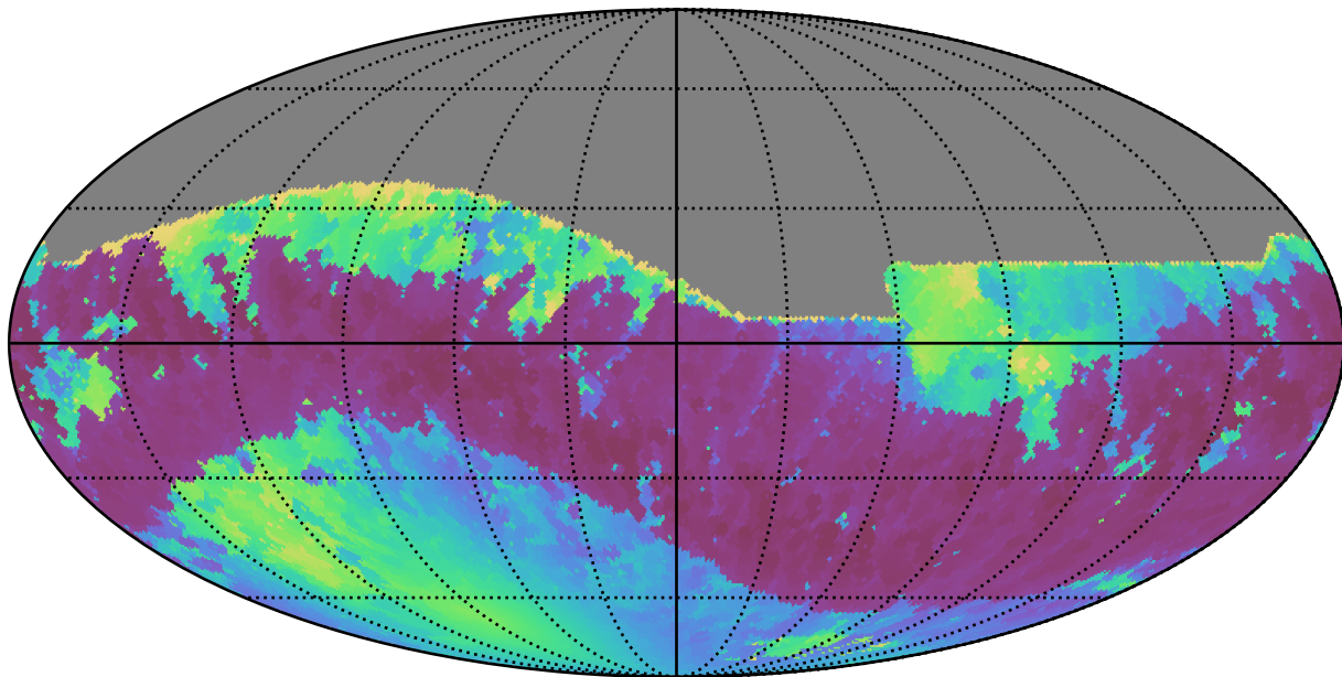
baseline_v3.5_10yrs All sky r band: Min solarElong
